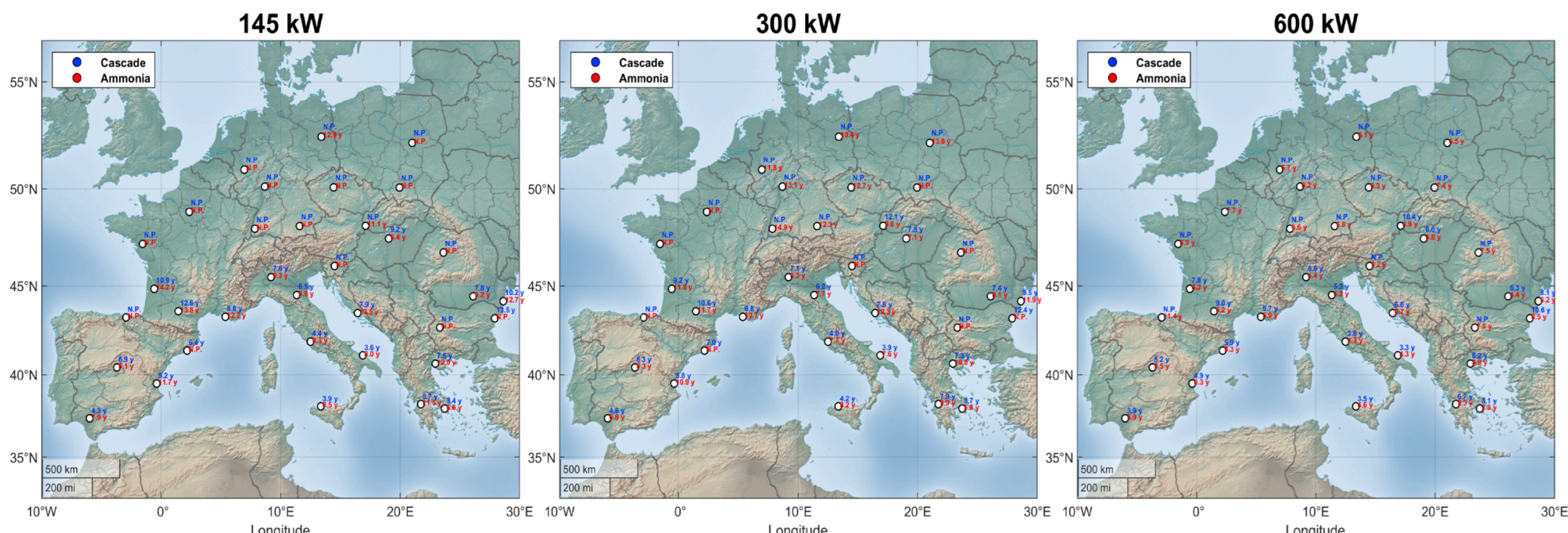
Figure 2. Simple payback of ammonia and cascade systems; N.P. indicates more than 15 years. Electricity prices: Eurostat non-household industrial band IC.
